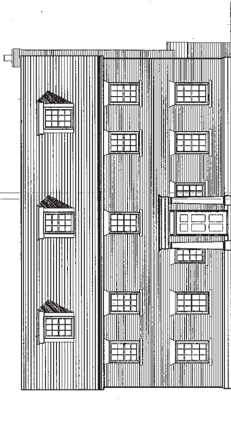
FRONT ELEVATION (EAST)
